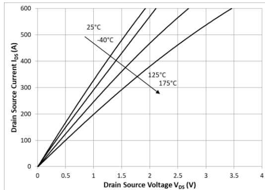
Figure 1: Drain current vs V_{DS} ( V_{GS}=15V , t_p < 200\mu s ) 7
