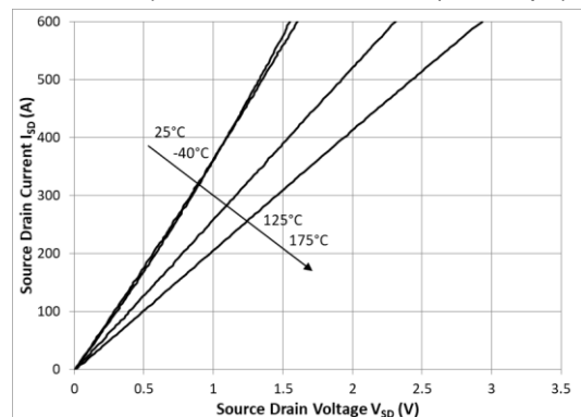
Figure 5: 3rd quadrant characteristics ( V_{GS}=15V , t_p < 200\mu s ) 7
