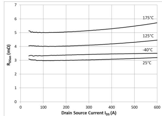
Figure 2: On-state drain source resistance vs. Drain current ( V_{GS}=15V , t_p < 200\mu s ) 7
