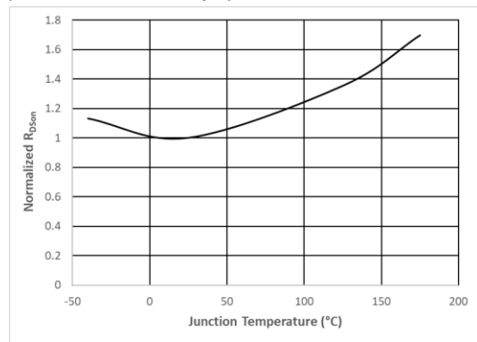
Figure 3: Normalized on-state drain source resistance ( I_{DS}=300A , V_{GS}=15V , t_p < 200\mu s ) 7
