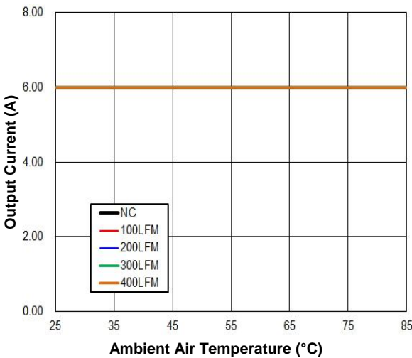
Figure 7. Derating Curve for Airflow Direction 1 (Ref. Figure. 8 for Airflow Direction; typical V_{in} , open frame, unit soldered onto a fixture board.)
