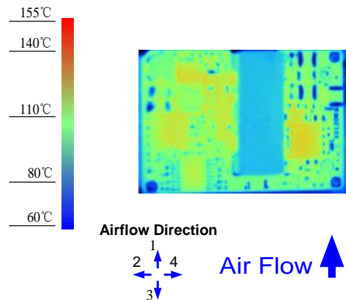
Figure 8. Thermal Image for Airflow Direction 1 (6A output, 55^{\circ}C ambient, 200LFM, typical V_{in} , open frame, unit soldered onto a fixture board.)
