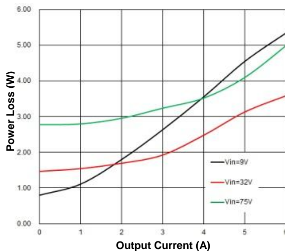
Figure 2. Power loss (25°C)
