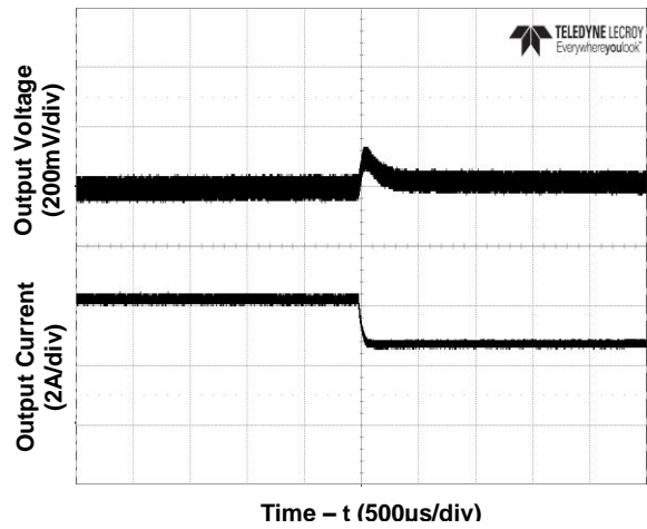
Figure 6. Transient Load Response (Typical V_{in} , 75% to 50% full load step at a slew rate 0.1A/\mu s )
