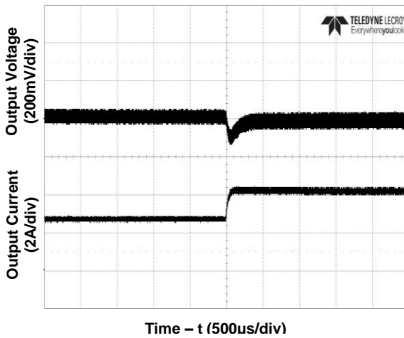
Figure 5. Transient Load Response (Typical V_{in} , 50% to 75% full load step at a slew rate 0.1A/\mu s )
