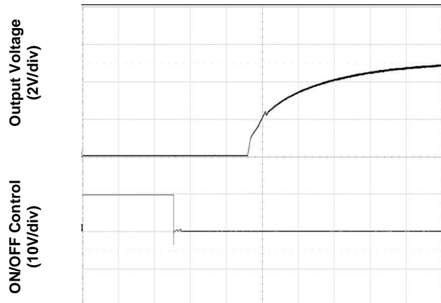
Figure 4. Start-Up from Enable Control (typical Vin)
