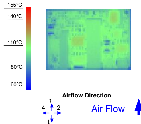
Figure 8. Thermal Image for Airflow Direction 3 (12.8A output, 55°C ambient, 200 LFM, typical Vin, open frame, unit soldered onto a fixture board)
