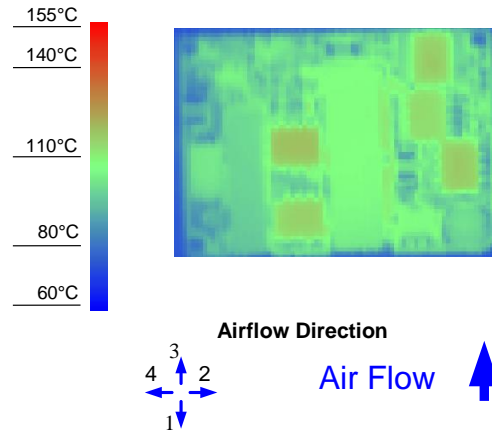
Figure 8. Thermal Image for Airflow Direction 3 (8A output, 55°C ambient, 0 LFM, typical Vin, open frame, unit soldered onto a fixture board)
