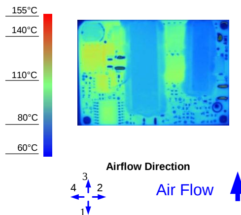
Figure 8. Thermal Image for Airflow Direction 3 (23A output, 55°C ambient, 200 LFM, typical Vin, open frame, unit soldered onto a fixture board)
