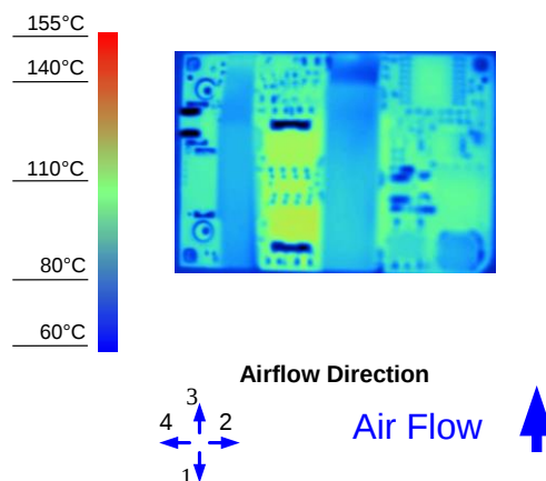
Figure 8. Thermal Image for Airflow Direction 3 (23.5A output, 55°C ambient, 200 LFM, typical Vin, open frame, unit soldered onto a fixture board)
