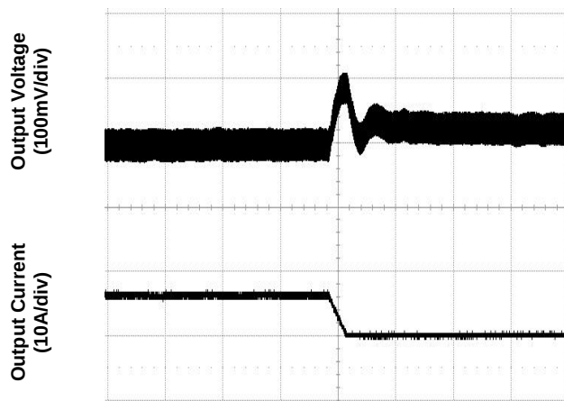
Figure 5. Transient Load Response (typical Vin, load current steps from 75% to 50% at a slew rate 0.1A/μs)
