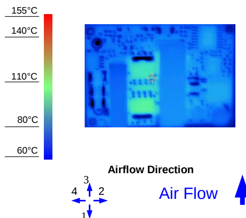
Figure 8. Thermal Image for Airflow Direction 3 (25A output, 55°C ambient, 0 LFM, typical Vin, open frame, unit soldered onto a fixture board)
