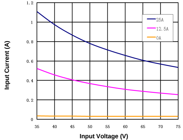
Figure 2. Input Characteristic (25°C)
