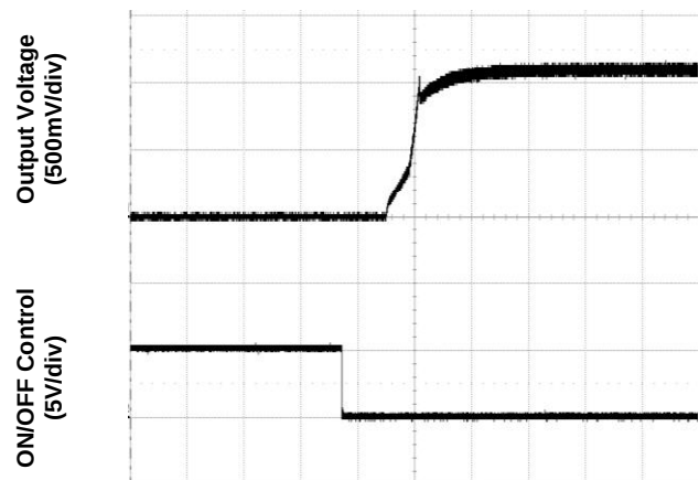
Figure 4. Start-Up from Enable Control (typical Vin, full load)
