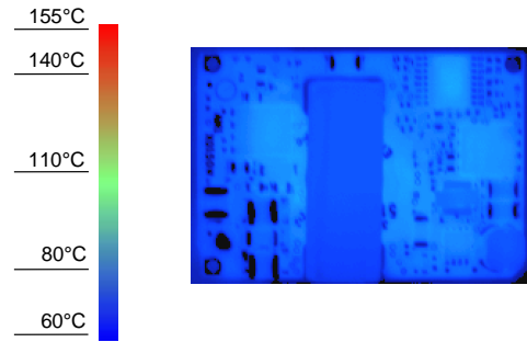
Figure 8. Thermal Image for Airflow Direction 3 (3A output, 55°C ambient, 200 LFM, typical Vin, open frame, unit soldered onto a fixture board)
