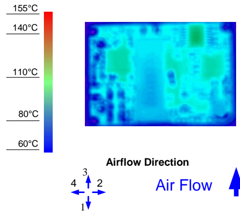
Figure 8. Thermal Image for Airflow Direction 3 (3A output, 55°C ambient, 200 LFM, typical Vin, open frame, unit soldered onto a fixture board)
