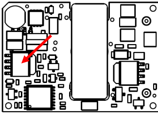
Figure 14. Temperature Monitoring Locations
