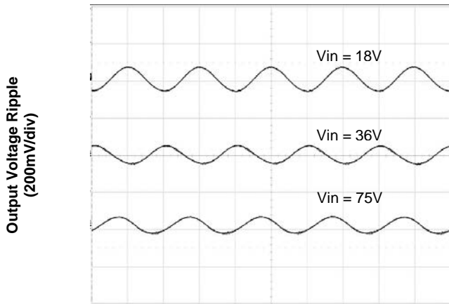
Figure 3. Output Ripple Voltage at Full Load
