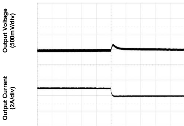
Figure 5. Transient Load Response (typical Vin, load current steps from 75% to 50% at a slew rate 0.1A/μs)
