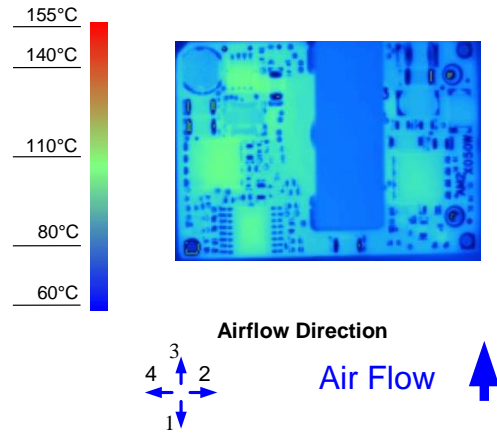
Figure 8. Thermal Image for Airflow Direction 3 (10A output, 55°C ambient, 200 LFM, typical Vin, open frame, unit soldered onto a fixture board)
