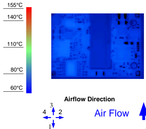
Figure 8. Thermal Image for Airflow Direction 3 (8A output, 55°C ambient, 200 LFM, typical Vin, open frame, unit soldered onto a fixture board)
