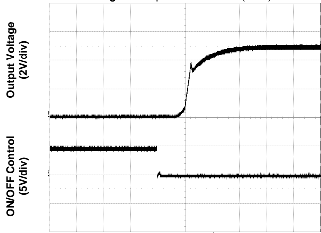
Figure 4. Start-Up from Enable Control (typical Vin, full load)
