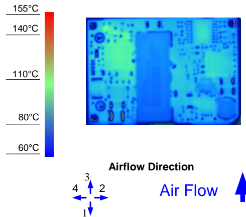
Figure 8. Thermal Image for Airflow Direction 3 (17.5A output, 55°C ambient, 200 LFM, typical Vin, open frame, unit soldered onto a fixture board)
