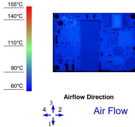
Figure 8. Thermal Image for Airflow Direction 3 (10A output, 55°C ambient, 200 LFM, typical Vin, open frame, unit soldered onto a fixture board)
