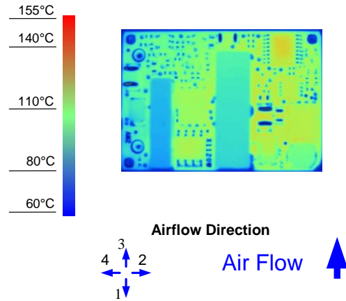
Figure 8. Thermal Image for Airflow Direction 3 (5A output, 55°C ambient, 200 LFM, typical Vin, open frame, unit soldered onto a fixture board)
