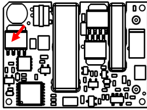
Figure 14. Temperature Monitoring Locations
