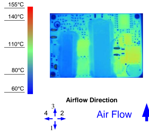
Figure 8. Thermal Image for Airflow Direction 3 (6.5A output, 55°C ambient, 200 LFM, typical Vin, open frame, unit soldered onto a fixture board)
