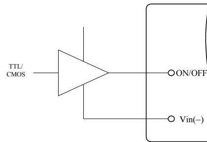
Figure 3. Direct Logic Drive
