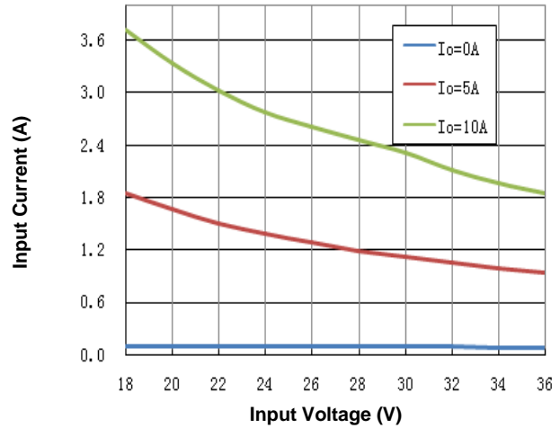
Figure 2. Input Characteristic (25°C)
