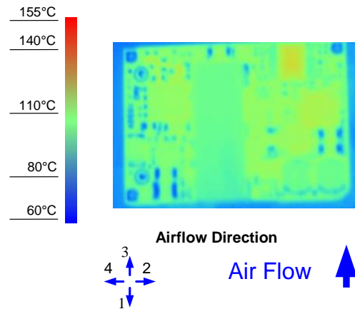
Figure 8. Thermal Image for Airflow Direction 3 (6A output, 55°C ambient, 200 LFM, typical Vin, open frame, unit soldered onto a fixture board)
