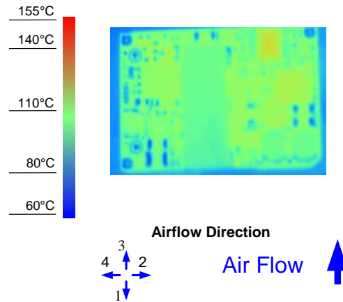
Figure 8. Thermal Image for Airflow Direction 3 (3A output, 55°C ambient, 200 LFM, typical Vin, open frame, unit soldered onto a fixture board)
