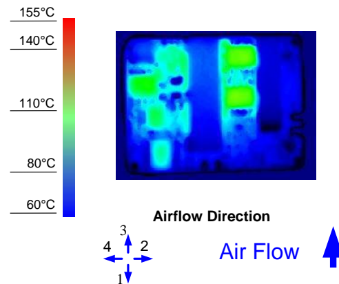
Figure 12. Thermal Image for Airflow Direction 3 (12A output, 55°C ambient, 200 LFM, typical V_{in} , open frame, unit soldered into fixture board)
