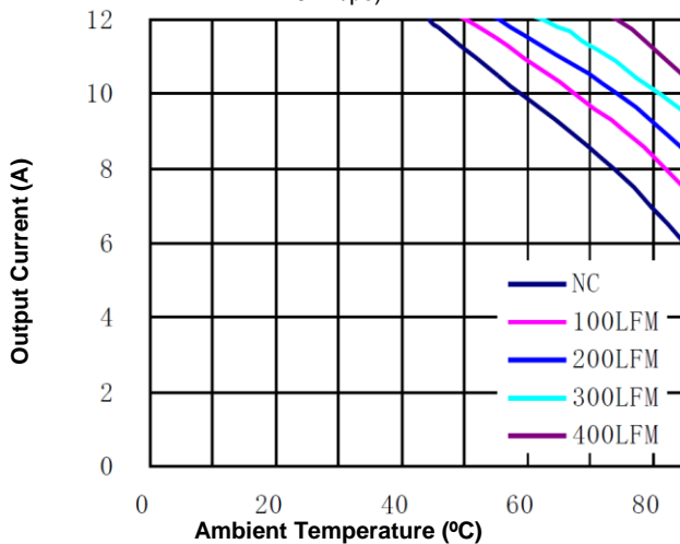
Figure 11. Derating Curve for Airflow Direction 3
