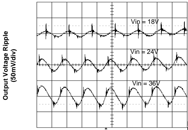
Figure 3. Output Voltage Ripple at Full Load
