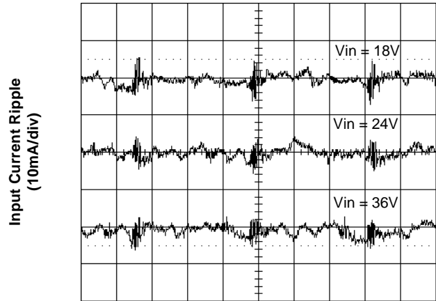
Figure 4. Input Reflected Ripple Current at Full Load
