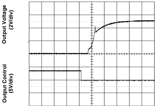
Figure 5. Start-Up from Enable Control (typical Input voltage and full load)
