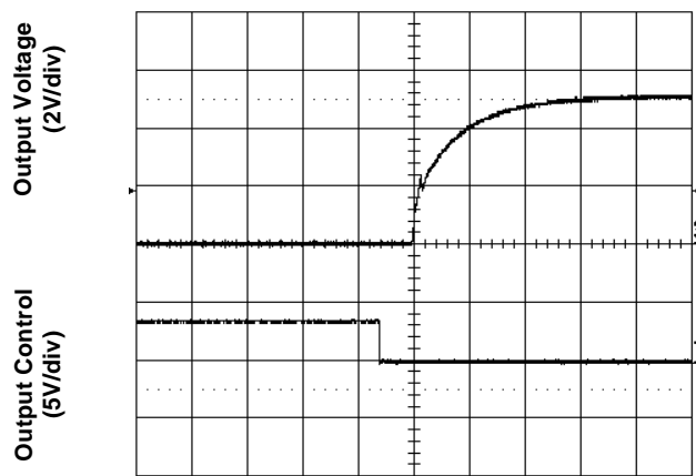
Figure 6. Start-Up from Enable Control (typical Input voltage and zero load)
