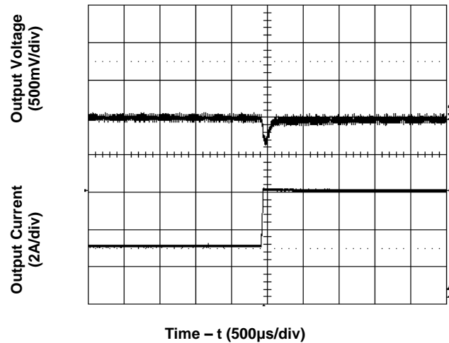
Figure 10. Transient Load Response
