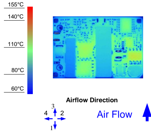
Figure 8. Thermal Image for Airflow Direction 3 (8A output, 55°C ambient, 200 LFM, typical Vin, open frame, unit soldered onto a fixture board)
