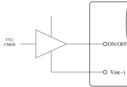
Figure 12. Direct Logic Drive
