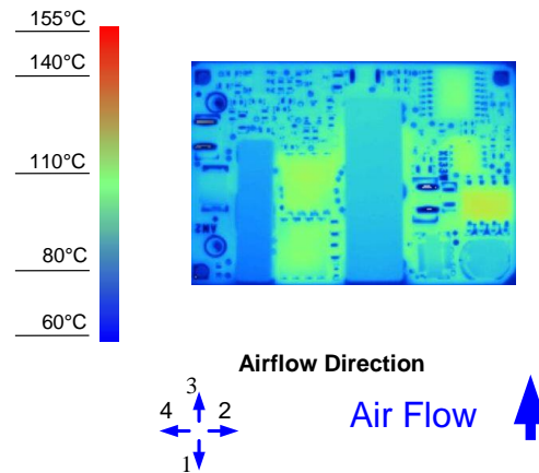
Figure 8. Thermal Image for Airflow Direction 3 (15A output, 55°C ambient, 200 LFM, typical Vin, open frame, unit soldered onto a fixture board)
