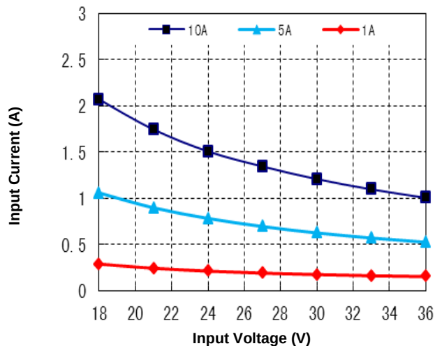
Figure 2. Input Characteristic (25°C)
