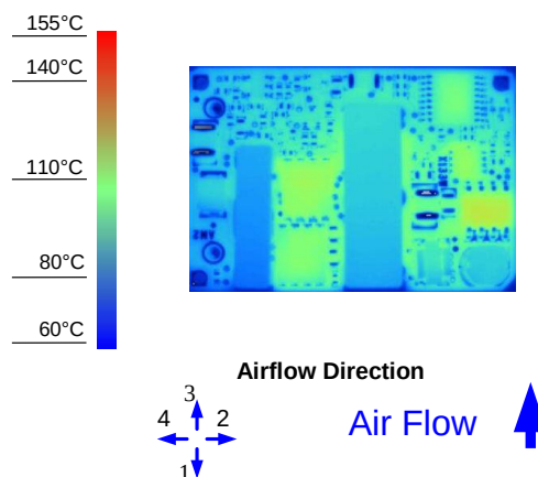
Figure 8. Thermal Image for Airflow Direction 3 (10A output, 55°C ambient, 200 LFM, typical Vin, open frame, unit soldered onto a fixture board)
