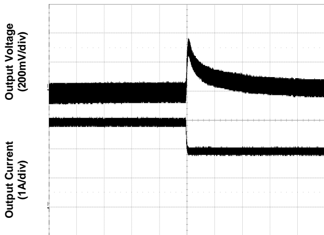
Figure 5. Transient Load Response (typical Vin, load current steps from 75% to 50% at a slew rate 0.1A/µs)
