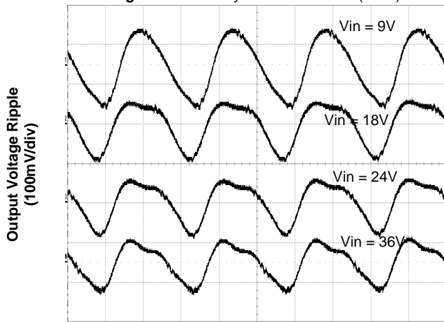
Figure 3. Output Ripple Voltage at Full Load
