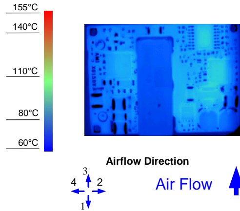
Figure 8. Thermal Image for Airflow Direction 3 (4A output, 55°C ambient, 200 LFM, typical Vin, open frame, unit soldered onto a fixture board)
