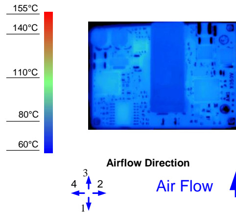
Figure 8. Thermal Image for Airflow Direction 3 (8A output, 55°C ambient, 200 LFM, V_{in} =18V, open frame, unit soldered onto a fixture board)
