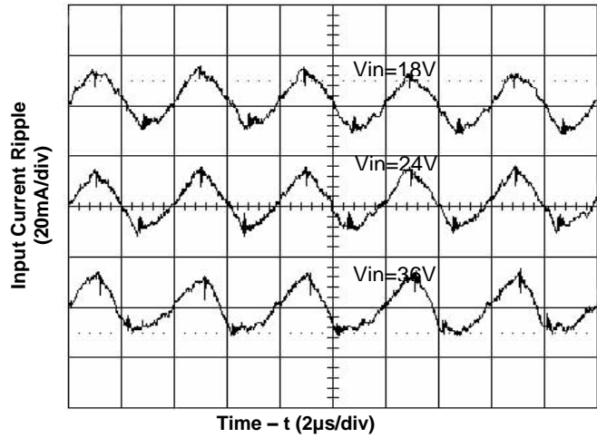
Figure 6. Input Reflected Ripple Current at Full Load
