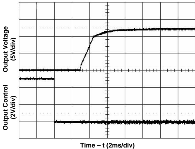
Figure 3. Start-Up from Enable Control Input voltage 24V, Output current 10A
