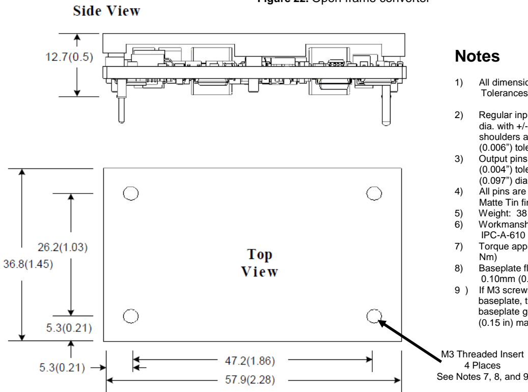
Figure 23. Converter with a baseplate
