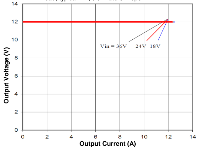
Figure 10. Output Characteristics
