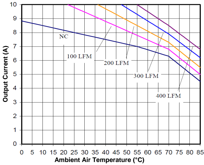
Figure 11. Current Derating Curve for Airflow Direction 3 (Ref. Fig. 12 for Airflow Direction; typical V_{in} , open frame unit using soldering interface)
