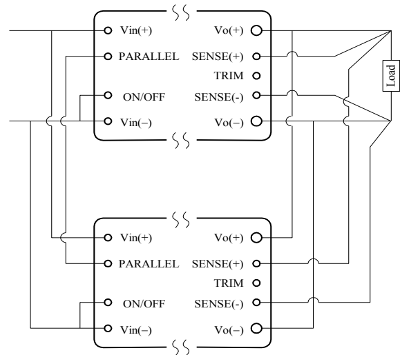
Figure 20. Circuit Configuration for Active Current Share
