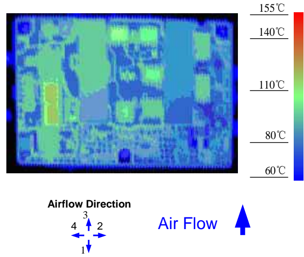
Figure 12. Thermal Image for Airflow Direction 3 (8.5A output, 55°C ambient, 200 LFM, typical V_{in} , open frame unit using soldering interface)
