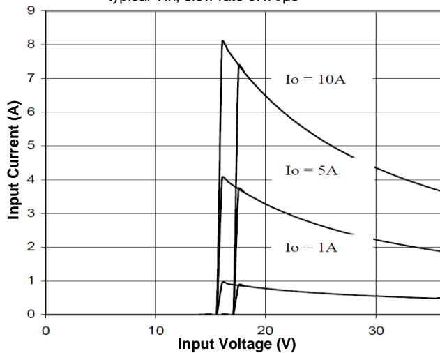
Figure 9. Input Characteristics
