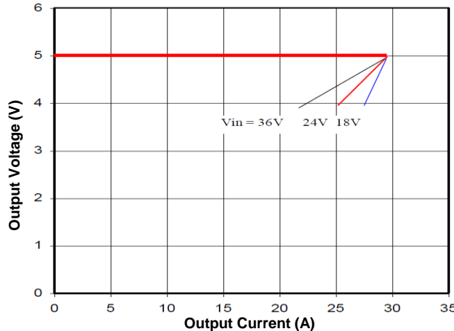
Figure 10. Output Characteristics
