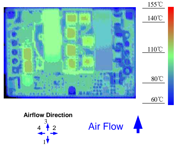
Figure 12. Thermal Image for Airflow Direction 3 (28A output, 55°C ambient, 200 LFM, typical V_{in} , open frame unit using soldering interface)
