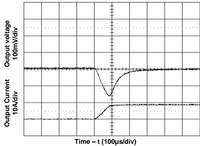
Figure 8. Transient Load Response Top: Output voltage deviation Bottom: Load current step (+25% full load) Test Cond.: Output current at 20A 50% full load, typical V_{in} , slew rate 0.1A/ \mu s
