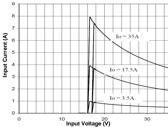
Figure 9. Input Characteristics
