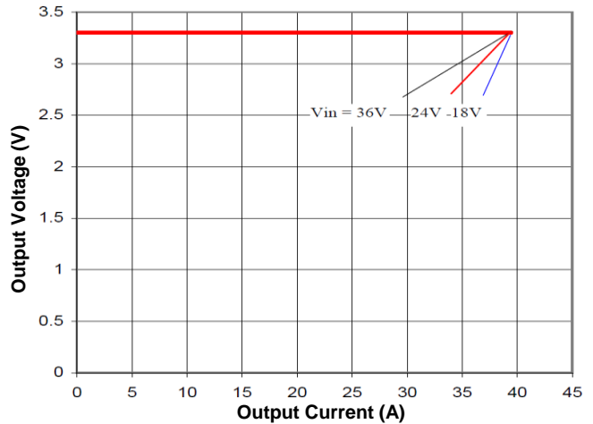
Figure 10. Output Characteristics
