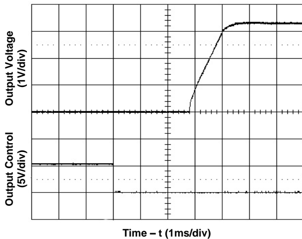
Figure 3. Start-Up from Enable Control Input voltage 24V, Output current 35A
