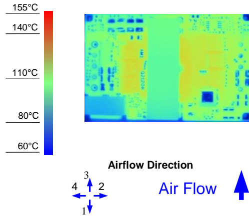
Figure 8. Thermal Image for Airflow Direction 3 (10A output, 55°C ambient, 200 LFM, typical Vin, open frame, soldered interface)
