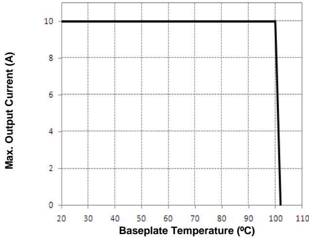
Figure 9. Current Derating Curve for Baseplate (typical Vin with baseplate, soldered interface)
