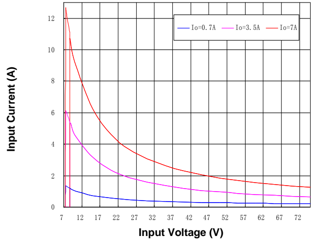
Figure 2. Input Characteristics (25°C)
