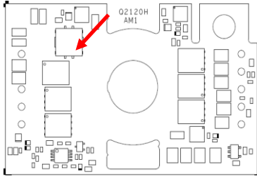
Figure 14. Temperature Monitoring Locations
