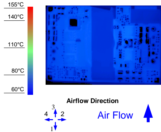
Figure 8. Thermal Image for Airflow Direction 3 (7A output, 55°C ambient, 200 LFM, typical Vin, open frame, soldered interface)
