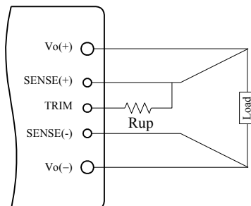
Figure 13. Circuit to Increase Output Voltage
