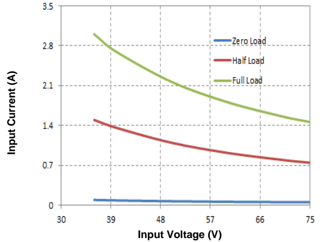
Figure 2. Input Characteristics (25°C)
