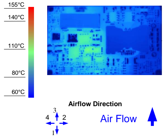
Figure 8. Thermal Image for Airflow Direction 3 (2A output, 55°C ambient, 200 LFM, typical Vin, open frame, soldered interface)
