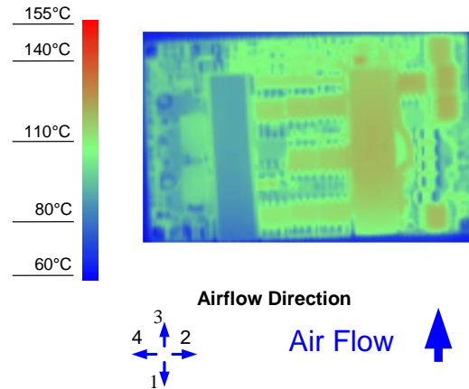
Figure 8. Thermal Image for Airflow Direction 3 (11.5A output, 55°C ambient, 200 LFM, typical Vin, open frame, soldered interface)
