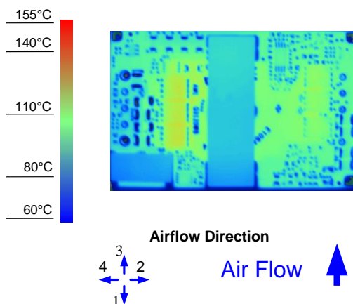
Figure 8. Thermal Image for Airflow Direction 3 (15A output, 55°C ambient, 200 LFM, typical Vin, open frame, soldered interface)
