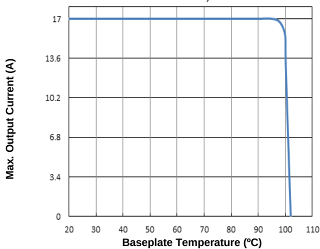
Figure 11. Current Derating Curve for Baseplate (typical V_{in} with baseplate, soldered interface)
