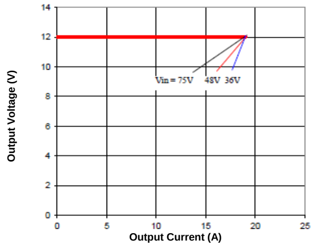
Figure 8. Output Characteristics (25°C)
