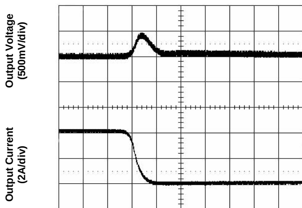
Figure 5. Transient Load Response (typical Vin, load current steps from 50% to 25% at a slew rate 0.1A/µs)
