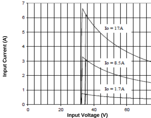
Figure 7. Input Characteristics (25°C)
