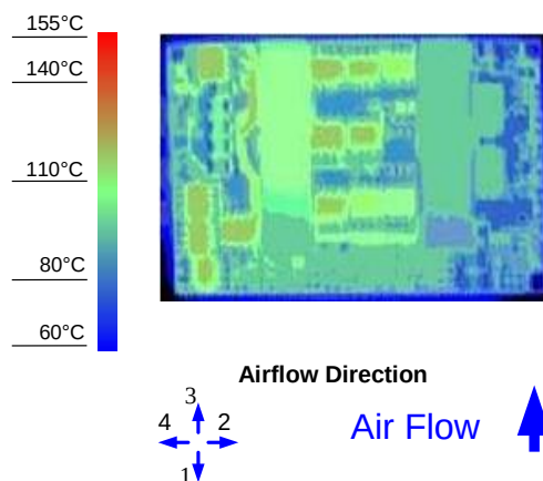
Figure 10. Thermal Image for Airflow Direction 3 (14.5A output, 55°C ambient, 200 LFM, typical V_{in} , open frame, soldered interface)
