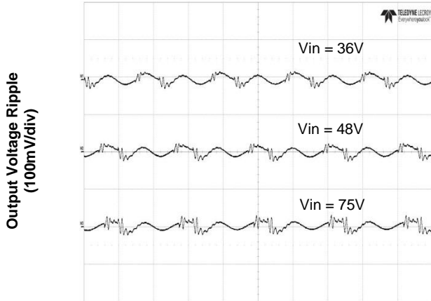
Time – t (2µs/div) Figure 3. Output Ripple Voltage at Full Load
