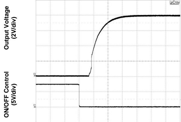
Time – t (5ms/div) Figure 4. Start-Up from Enable Control (typical Vin, full load)
