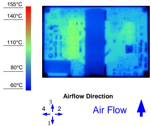
Figure 8. Thermal Image for Airflow Direction 3 (22A output, 55°C ambient, 200 LFM, typical Vin, open frame, unit soldered onto a fixture board)
