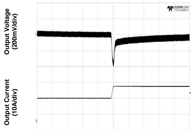
Time – t (500µs/div) Figure 6. Transient Load Response (typical Vin, load current steps from 50% to 75% at a slew rate 0.1A/µs)
