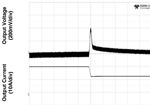
Time – t (500µs/div) Figure 5. Transient Load Response (typical Vin, load current steps from 75% to 50% at a slew rate 0.1A/µs)
