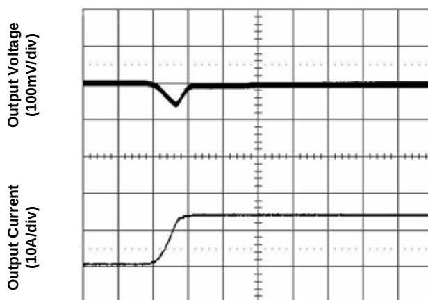
Figure 6. Transient Load Response (typical Vin, load current steps from 50% to 75% at a slew rate 0.1A/μs)
