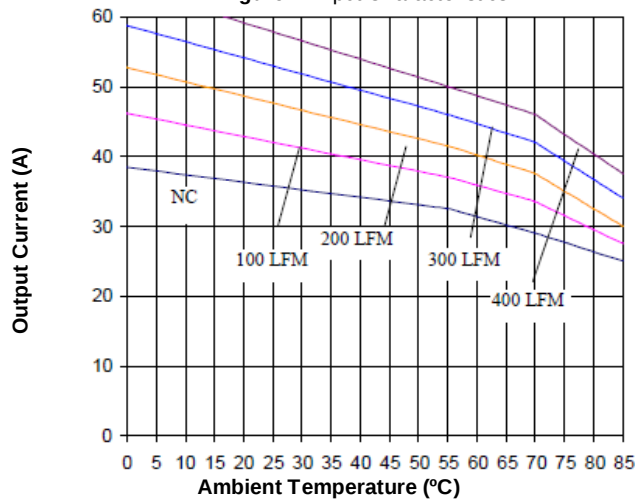
Figure 9. Current Derating Curve for Airflow Direction 3 (Ref. Fig. 10 for Airflow Direction; typical V_{in} , open frame, soldered interface)
