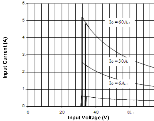
Figure 7. Input Characteristics
