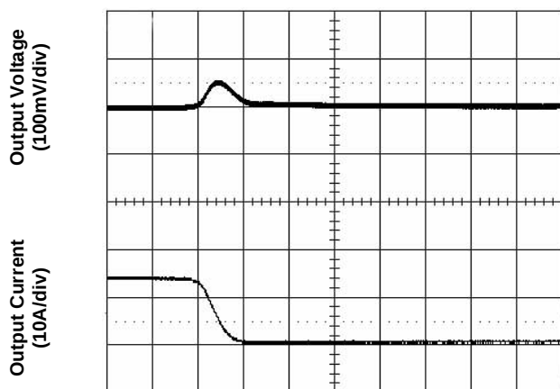
Figure 5. Transient Load Response (typical Vin, load current steps from 50% to 25% at a slew rate 0.1A/μs)
