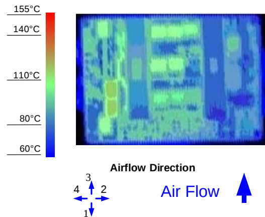
Figure 10. Thermal Image for Airflow Direction 3 (41.5A output, 55 ^{\circ}C ambient, 200 LFM, typical V_{in} , open frame, soldered interface)
