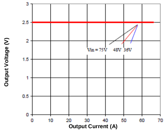
Figure 8. Output Characteristics
