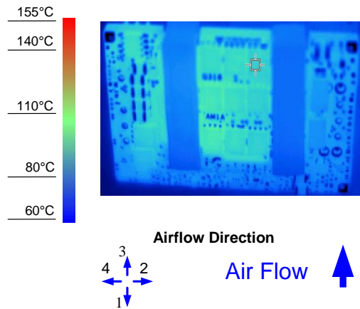
Figure 10. Thermal Image for Airflow Direction 3 (80A output, 55°C ambient, 200 LFM, typical Vin, open frame, soldered interface)
