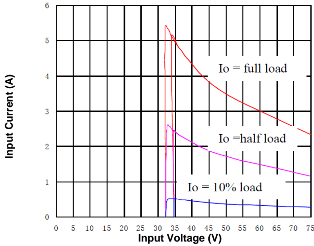
Figure 7. Input Characteristics
