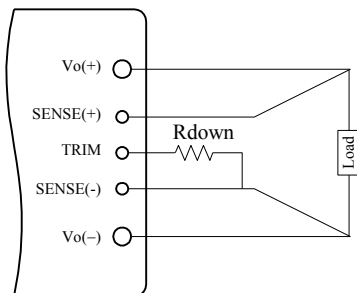
Figure 14. Circuit to Decrease Output Voltage
