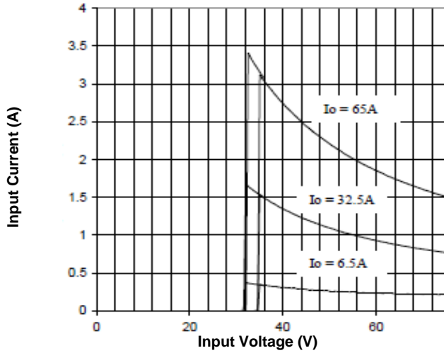
Figure 7. Input Characteristics
