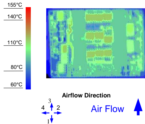
Figure 10. Thermal Image for Airflow Direction 3 (50A output, 55°C ambient, 200 LFM, typical V_{in} , open frame, soldered interface)
