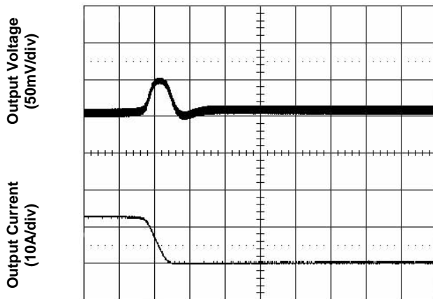
Figure 5. Transient Load Response (typical V_{in} , load current steps from 50% to 25% at a slew rate 0.1A/ \mu s)
