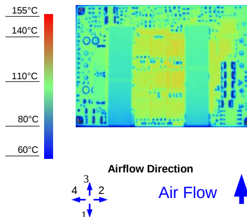
Figure 8. Thermal Image for Airflow Direction 3 (93A output, 55°C ambient, 200 LFM, typical Vin, open frame, soldered interface)
