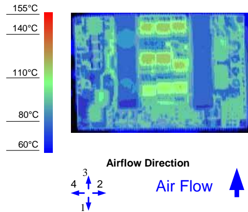
Figure 10. Thermal Image for Airflow Direction 3 (58.5A output, 55°C ambient, 200 LFM, typical V_{in} , open frame, soldered interface)
