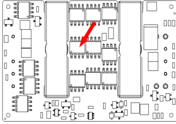
Figure 17. Temperature Monitoring Locations
