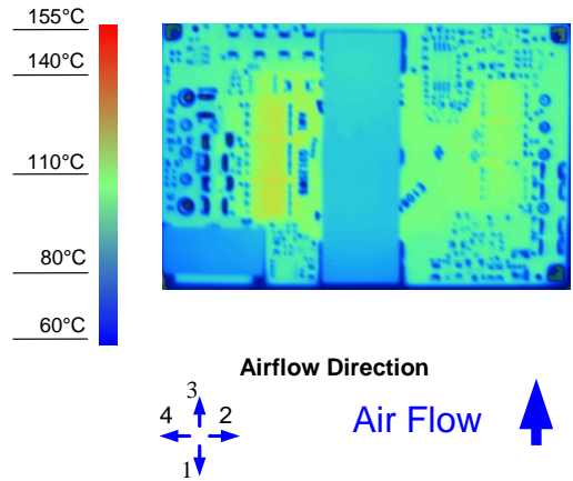
Figure 8. Thermal Image for Airflow Direction 3 (14A output, 55°C ambient, 200 LFM, typical Vin, open frame, unit soldered onto a fixture board)
