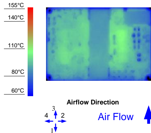
Figure 8. Thermal Image for Airflow Direction 3 (25A output, 55°C ambient, 200 LFM, typical Vin, open frame, unit soldered onto a fixture board)
