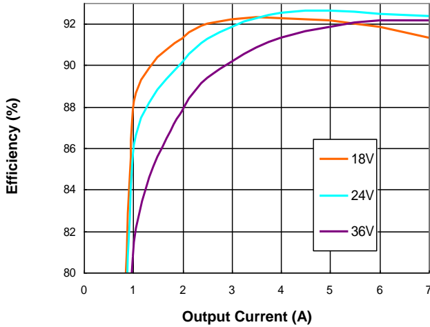
Figure 1. Efficiency vs. Load Current (25°C)
