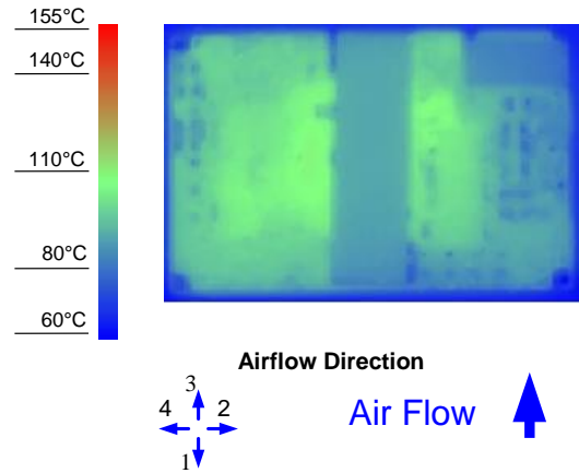
Figure 8. Thermal Image for Airflow Direction 3 (5.6A output, 55°C ambient, 200 LFM, typical Vin, open frame, soldered interface)
