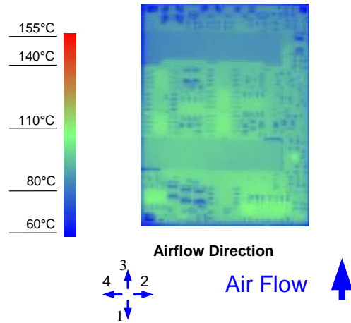
Figure 8. Thermal Image for Airflow Direction 3 (4.3A output, 55°C ambient, 200 LFM, typical Vin, open frame, soldered interface)
