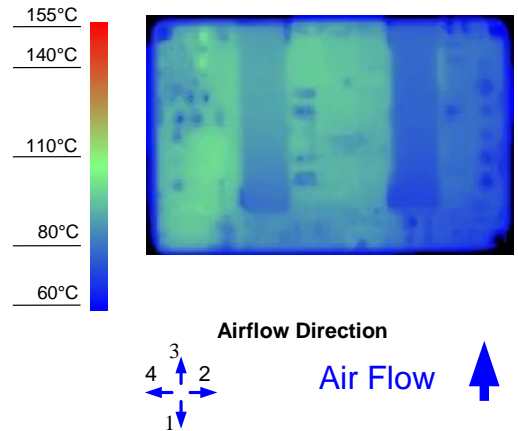
Figure 8. Thermal Image for Airflow Direction 3 (17A output, 55°C ambient, 200 LFM, typical Vin, open frame, unit soldered onto a fixture board)
