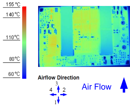
Figure 12. Thermal Image for Airflow Direction 3 (34.5A output, 55°C ambient, 200 LFM, typical V_{in} , open frame, soldered interface)
