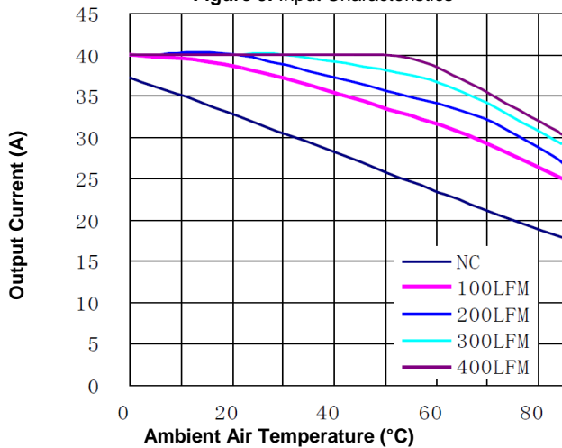
Figure 11. Current Derating Curve for Airflow Direction 3
