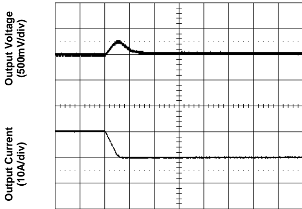
Time - t (200μs/div)
