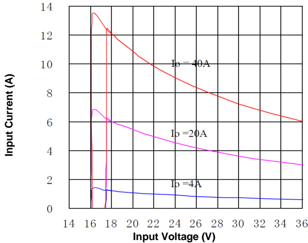
Figure 9. Input Characteristics
