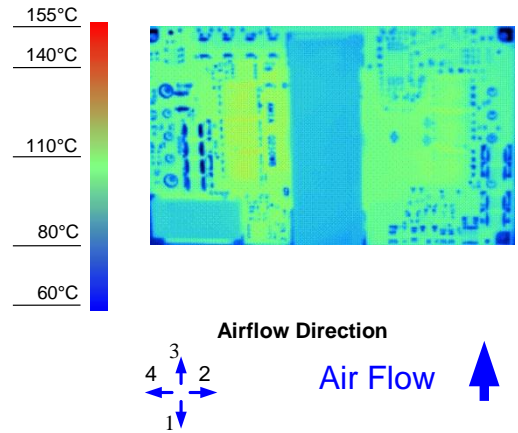
Figure 8. Thermal Image for Airflow Direction 3 (25A output, 55°C ambient, 200 LFM, typical Vin, open frame, unit soldered onto a fixture board)
